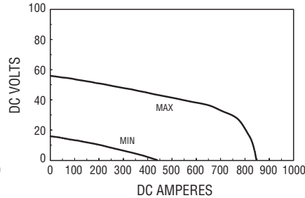
402/502 CC/CV VOLT/AMP CURVES – TIG MODE
