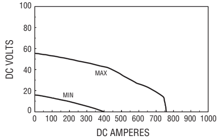
302 CC/CV VOLT/AMP CURVES – TIG MODE
