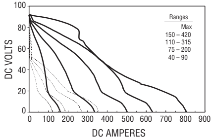
302 CC/CV VOLT/AMP CURVES – MIG MODE
