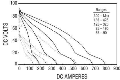
402/502 CC/CV VOLT/AMP CURVES – MIG MODE
